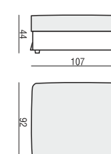
FOOTSTOOL 107x92
